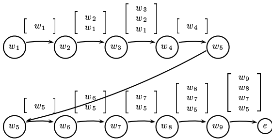
Figure 4: Propagating the head stack feature along the path.
